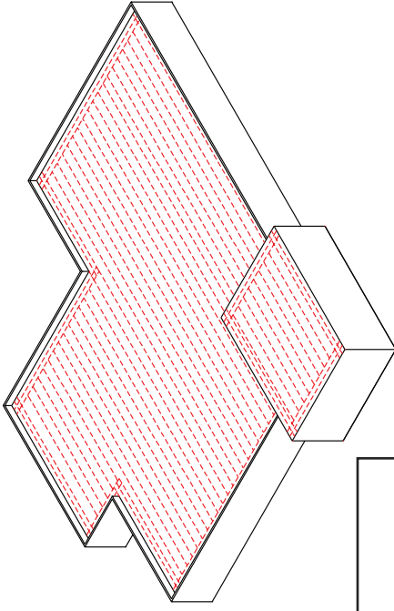
6' Wide Roll-Good Systems Linear Feet of Field Seams – 7,968
