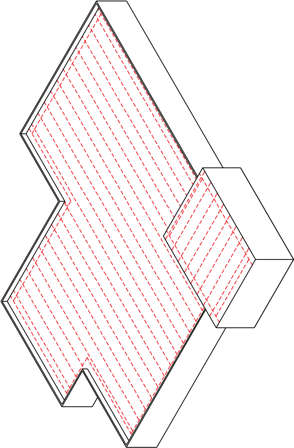
10' Wide Roll-Good Systems Linear Feet of Field Seams – 5,130
